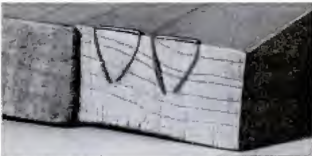
Chisel points on staple legs bring legs together with a light clinching action as they enter work
